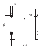
Installation Dimensions
