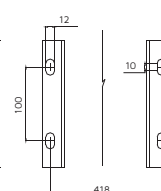
Installation Dimensions
