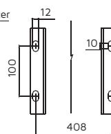
Installation Dimensions
