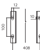
Installation Dimensions
